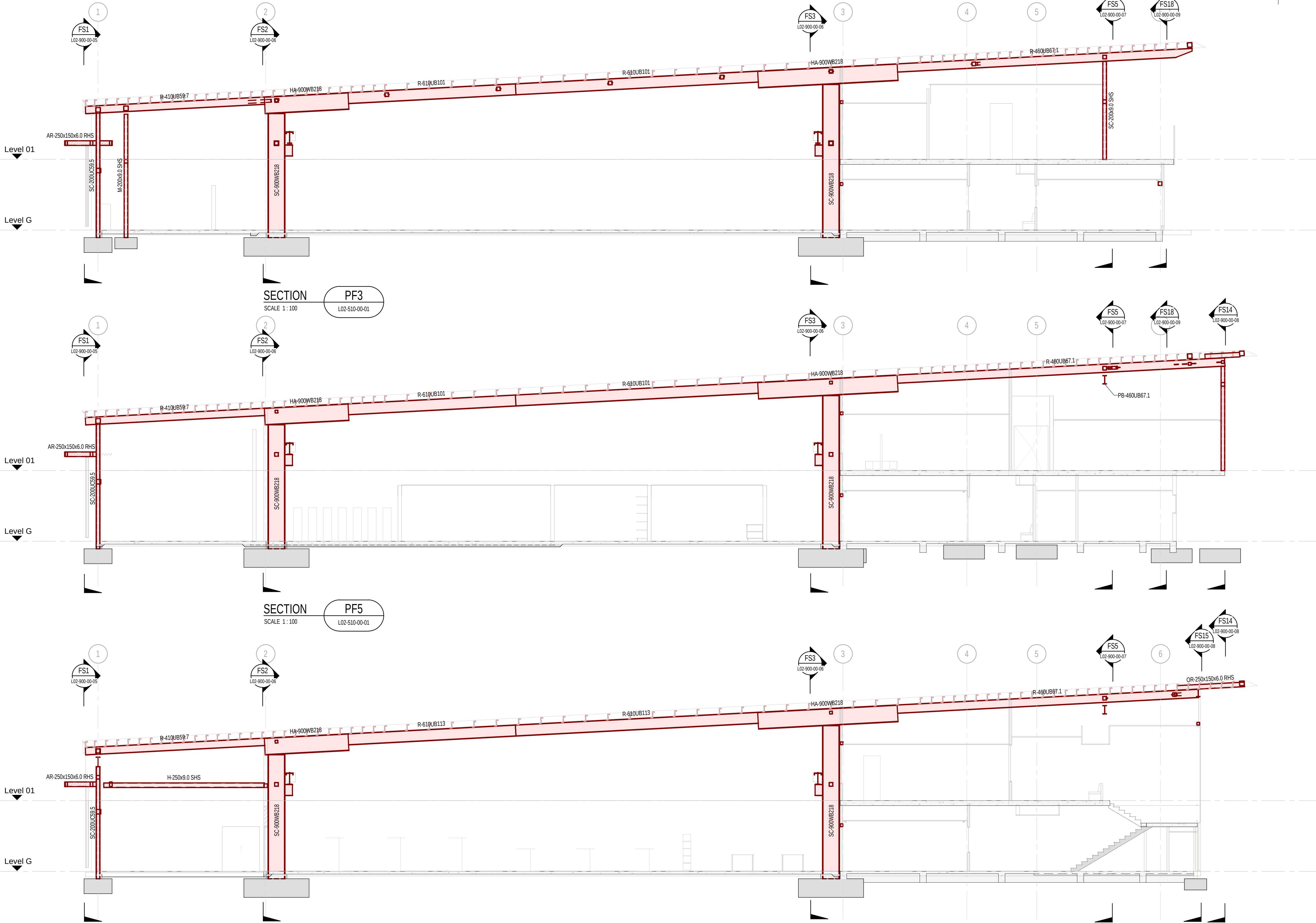
SECTION SCALE 1:100
